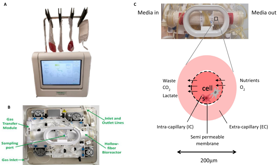
Figure 1. (A) The Quantum Cell Expansion System. (B) A single-use cassette, including the hollow-fiber bioreactor is inserted inside the Quantum Cell Expansion System, with the reactor connected to a gas supply and tubing inserted into the peristaltic pump system to move culture media through the system. (C) Schematic depicting the hollow fiber perfusion system inside the bioreactor, indicating the flow of nutrients, waste, CO 2 , O 2 and lactate across the semi-permeable membrane of the fibers.
